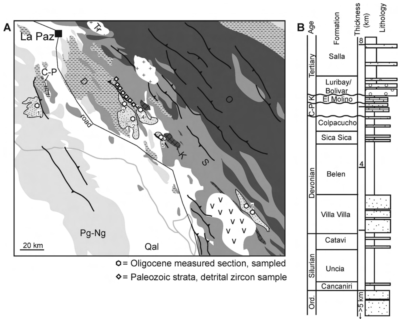
FIG. 2.—Geology of the study area and stratigraphy in the region. A ) Simplified geologic map of the study area showing lithologic units and prominent structural features. White hexagons mark specific study locations, and diamonds mark locations where samples of Paleozoic strata were sampled. Upper Oligocene exposures are denoted by Pg-Ng and have black outlines. Locations: 1 = Coro Coro, 2 = Salla, 3 = Luribay, 4 = North Puchuni, 5 = South Puchuni, 6 = Bolivar. Qal = Quaternary alluvium; Pg-Ng = Paleogene–Neogene sedimentary strata; V = Cenozoic volcanic strata; K = Cretaceous sedimentary strata; Tr = Triassic granite; C-P = Carboniferous–Permian sedimentary strata; D = Devonian sedimentary strata; S = Silurian sedimentary strata; O = Ordovician sedimentary strata. B ) Stratigraphy in the region with general thickness and lithology. Stippled pattern = sandstone; white = mudstone; brick = limestone; large circles = conglomerate.
