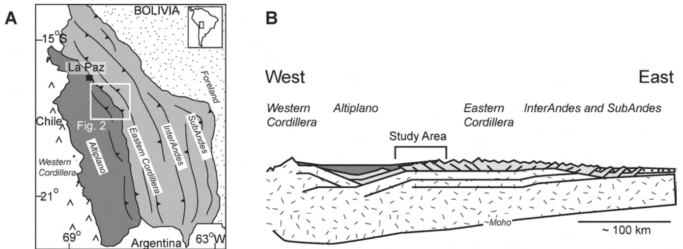
FIG. 1.—Location map and tectonic zones of the Central Andes. A ) Location map of study area showing the tectonic zones discussed in text. The Altiplano is shown in dark gray, the fold-thrust belt is in light gray, and the foreland in white. Location of Figure 2 is shown with a white box. B ) Schematic crustal-scale cross section through the Central Andes. The Altiplano is located between the Western Cordillera (modern arc) and the Huarina backthrust belt (west-vergent structures) of the Eastern Cordillera.
