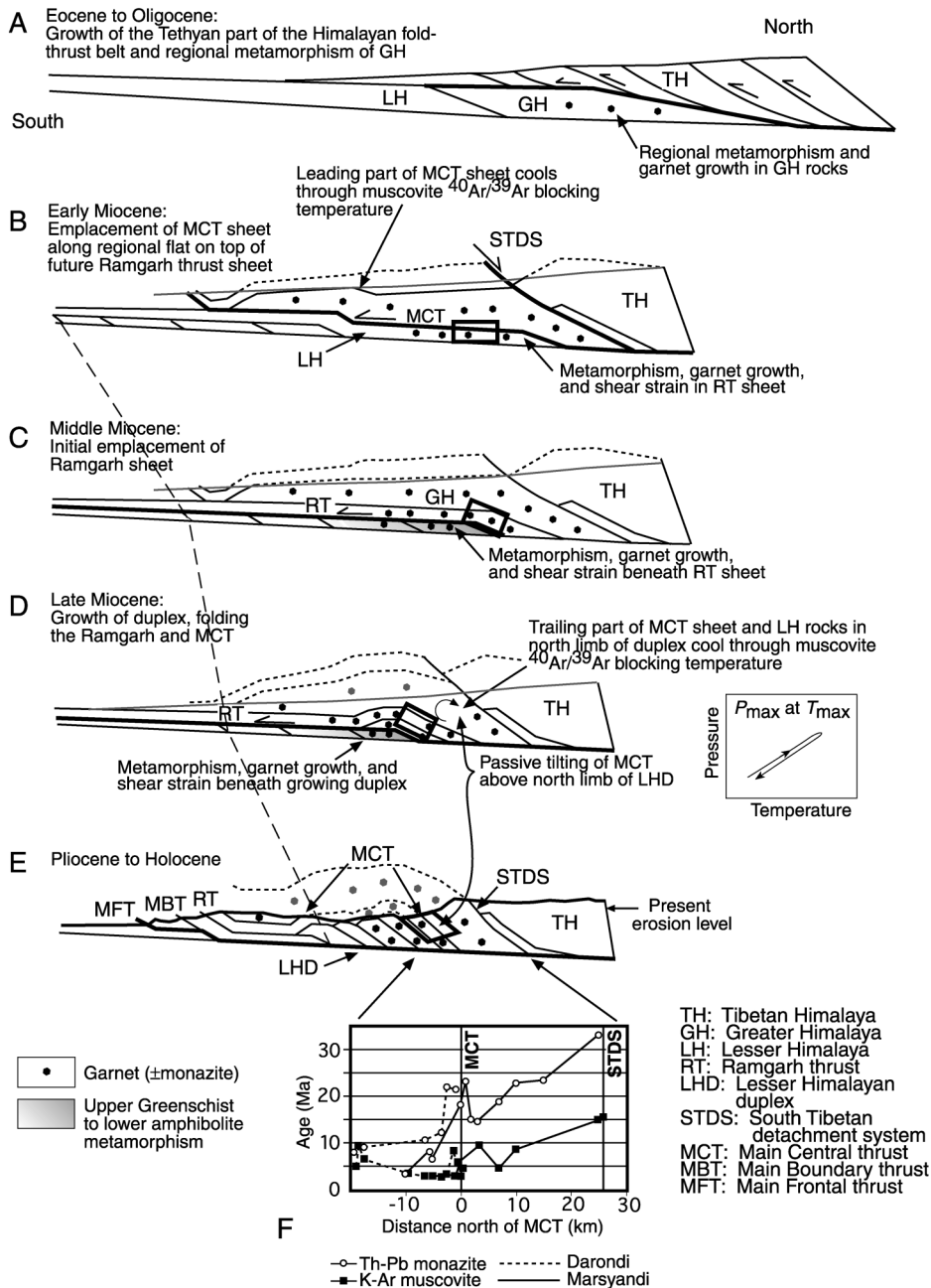
Figure 2. A–E: Evolution of Himalayan thrust belt beginning in early Tertiary time. Bold lines mark active fault(s). Polygon highlights part of Main Central thrust currently exposed at surface. Lines of long dashes connecting B–E track location of reference point. D: Schematic pressure-temperature ( P , T ) path for each thrust sheet in duplex (after Kohn et al., 2001). F: Th-Pb monazite and ^{40}\text{Ar}/^{39}\text{Ar} muscovite ages plotted against distance of samples from trace of Main Central thrust, from Darondi and Marsyandi Kholas in central Nepal (after Catlos et al., 2001). Location of sample area is shown in Figure 1A. Arrows indicate approximate distribution of ages relative to schematic model.
